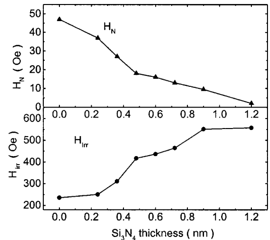
FIG. 2. The nucleation field H_N of the soft NiFe layer and the irreversible switching field H_{\text{irr}} of the hard SmFe layer versus the nonmagnetic insulating \text{Si}_3\text{N}_4 layer thickness for \text{Ni}_{80}\text{Fe}_{20} (63 nm)/ \text{Si}_3\text{N}_4 /Sm _{40}\text{Fe}_{60} (78 nm) sandwiches.
