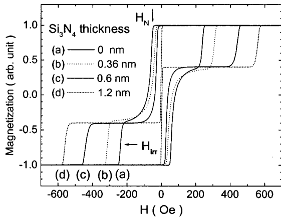
FIG. 1. Some typical easy-axis magnetization hysteresis loops of \text{Ni}_{80}\text{Fe}_{20} (63 nm)/ \text{Si}_3\text{N}_4 /Sm _{40}\text{Fe}_{60} (78 nm) sandwiches with various \text{Si}_3\text{N}_4 thicknesses. The thicknesses of the nonmagnetic insulating \text{Si}_3\text{N}_4 layer are (a) 0, (b) 0.36, (c) 0.6, and (d) 1.2 nm, respectively. The nucleation field H_N of the magnetically soft layer and the irreversible switching field H_{\text{irr}} of the magnetically hard layer are marked for Fig. 1(a).
