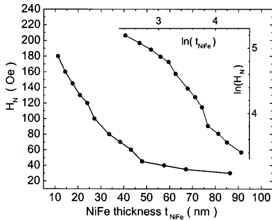
FIG. 3. The nucleation field H_N of the soft NiFe layer vs the NiFe layer thickness t for the \text{Ni}_{80}\text{Fe}_{20} (10–86 nm)/ \text{Si}_3\text{N}_4 (0.36 nm)/ \text{Sm}_{40}\text{Fe}_{60} (81.4 nm) sandwiches. The inset shows the dependence of \ln(H_N) on \ln(t) .
